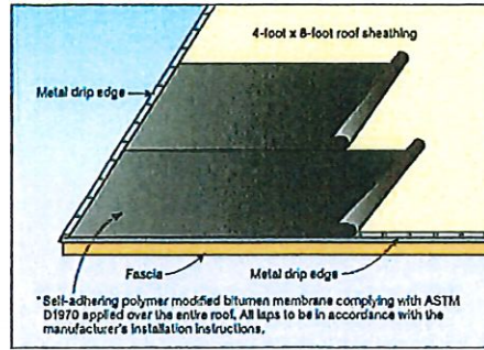
Sealed Roof Deck Option #1
