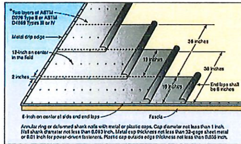
Sealed Roof Deck Option #3
