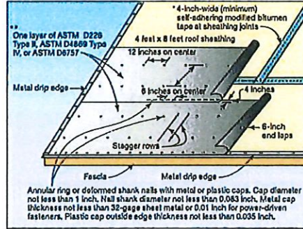
Sealed Roof Deck Option #2
